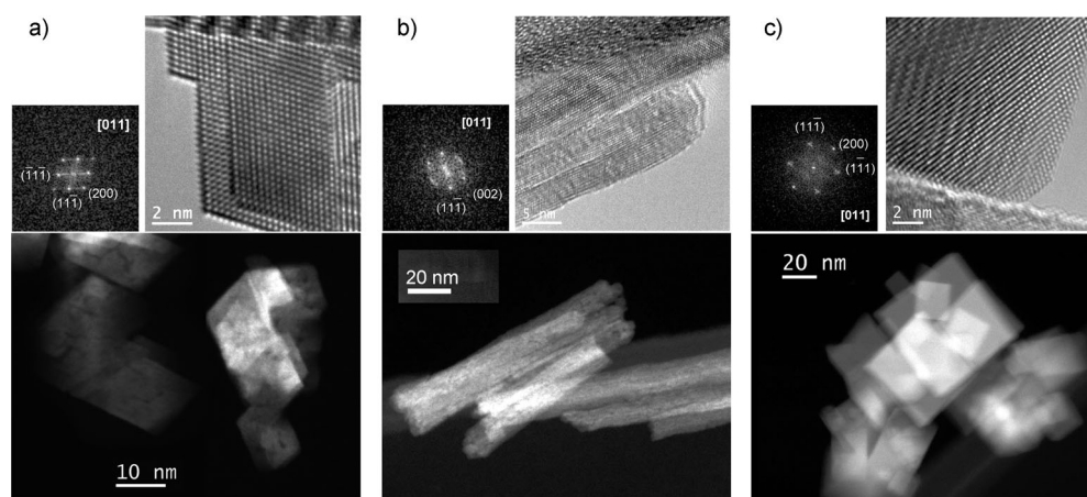
Figure 2. TEM images of the three CeO 2 nanostructures: a) Octahedra, b) Rods, and c) Cubes.
