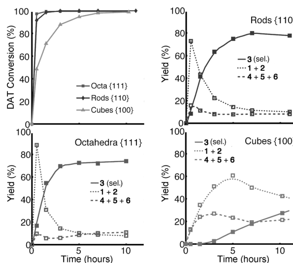
Figure 3. Carbamoylation of DAT over CeO 2 nanostructures. Conversion and yield of dicarbamoylated DAT (—), monocarbamoylated DAT (.....) and methylated products (---) obtained using nano-octahedra, nanorods, and nanocubes of CeO 2 as catalyst.
